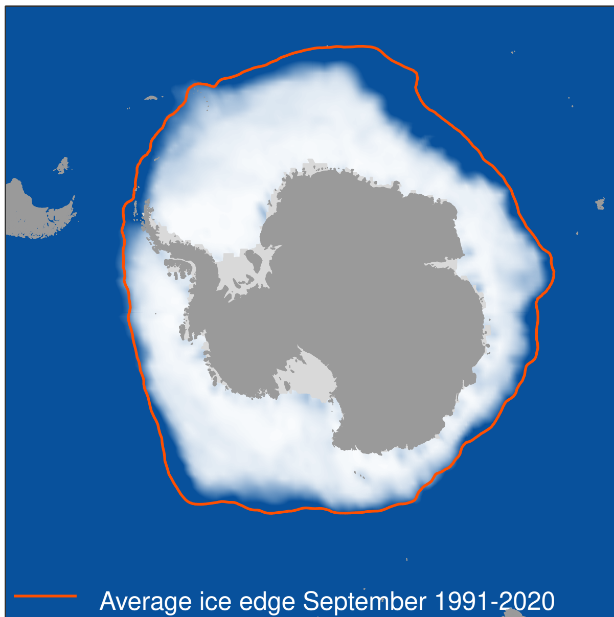
Average concentration
