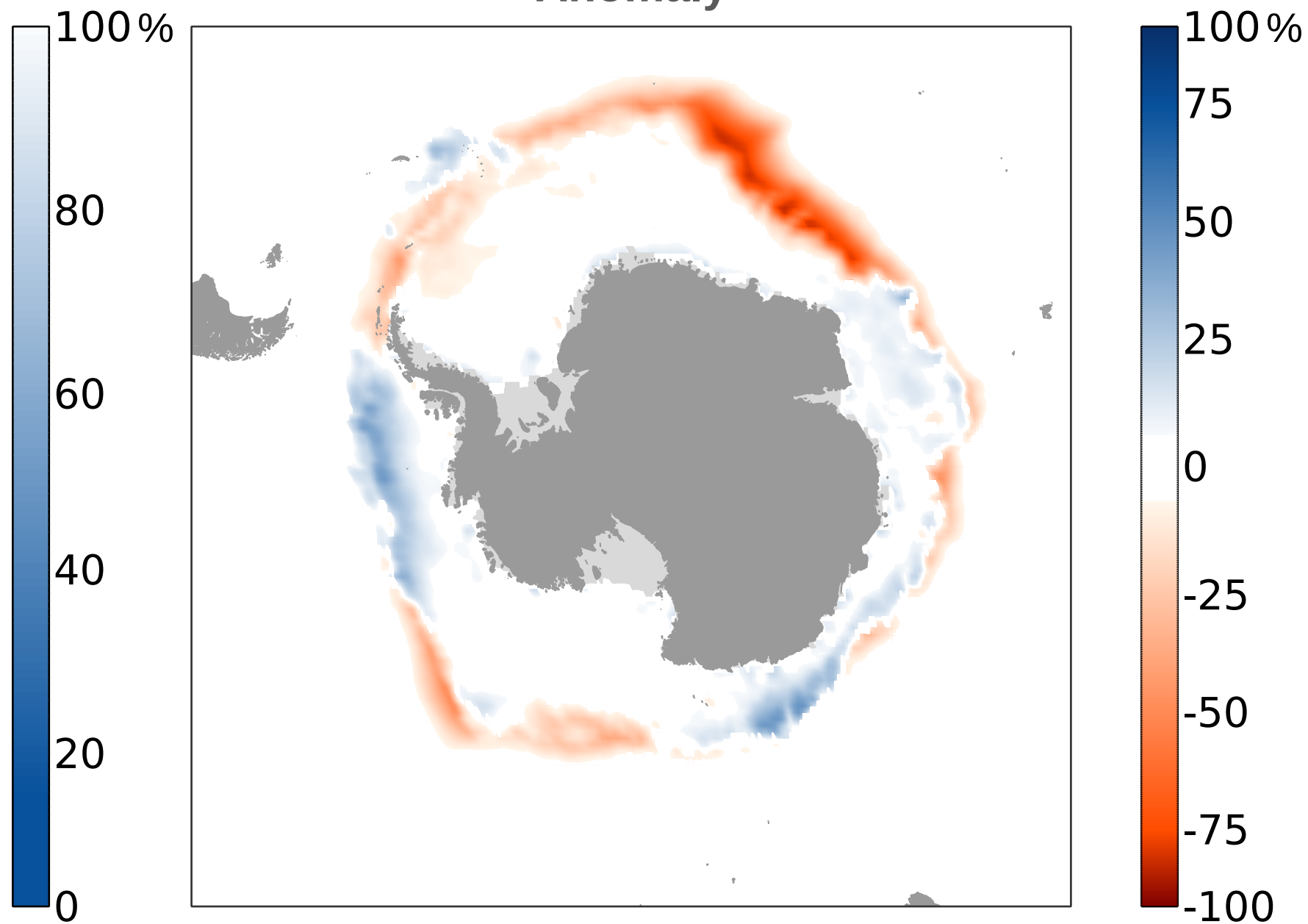
Anomaly
