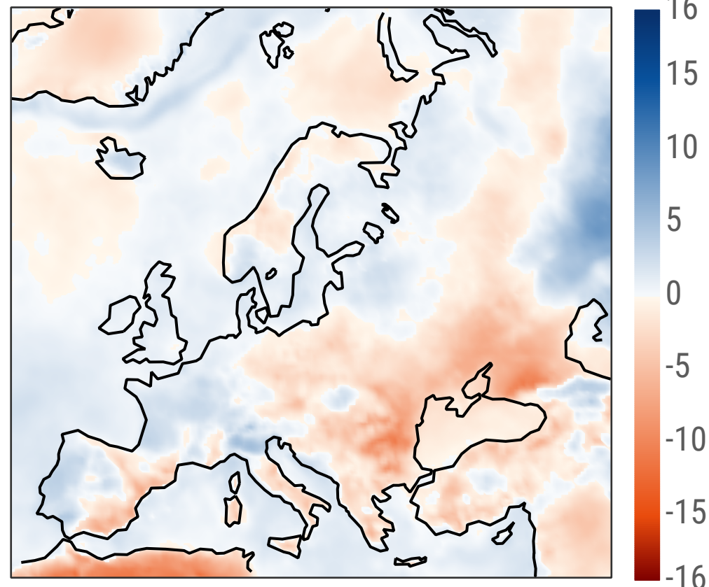
Surface air relative humidity (%)
