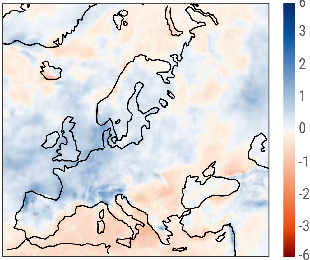
Precipitation (mm/day)
