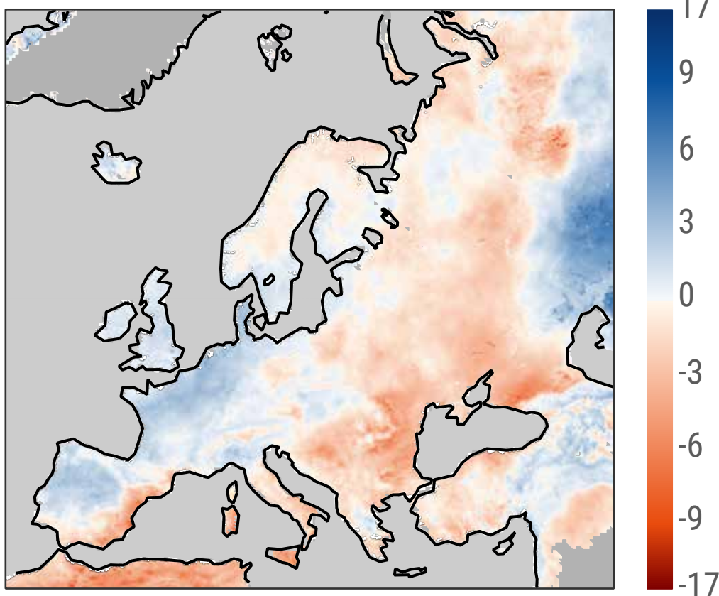
0-7cm volumetric soil moisture (%)
